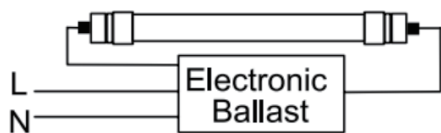
TYPE A(Ballast compatible)
