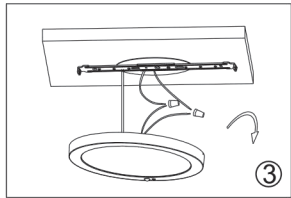
③ Connecting the wire;
