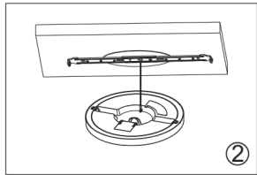
② Install the safe wire, lock one side on the bracket, another side on the light;
